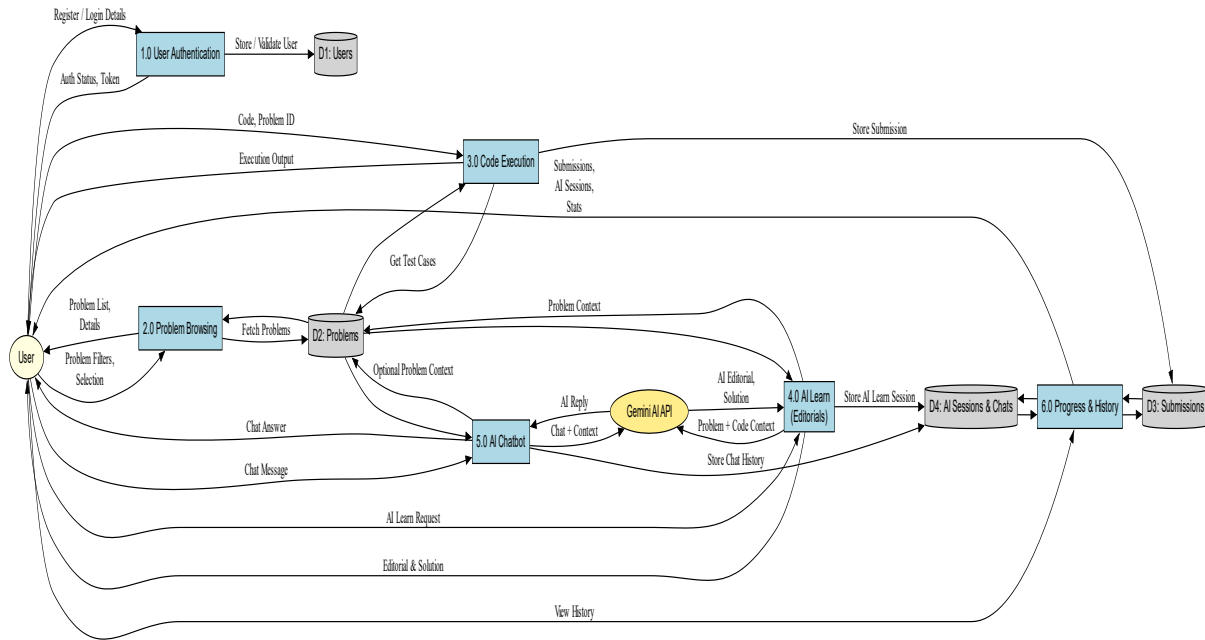
Figure 3.4 – Level 1 DFD for CodeCrash.AI
