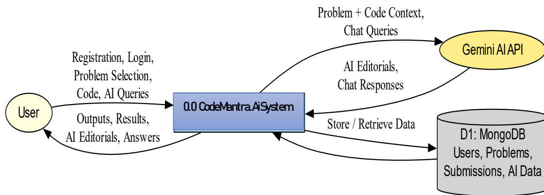
Figure 3.3 – Level 0 DFD for CodeMantra.AI
